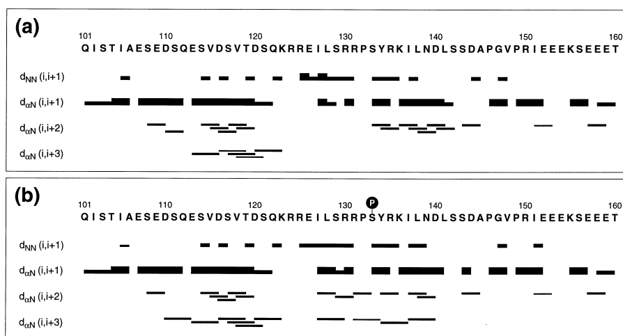
Fig. 4. NOE connectivity diagram summarizing sequential and medium-range correlations observed in 3D ^{15}\text{N} -edited NOESY ( \tau_m = 150 ms) spectra of the (a) non-phosphorylated and (b) Ser ^{133} -phosphorylated forms of KID. The thickness of the bars reflects the intensity of the correlations.
