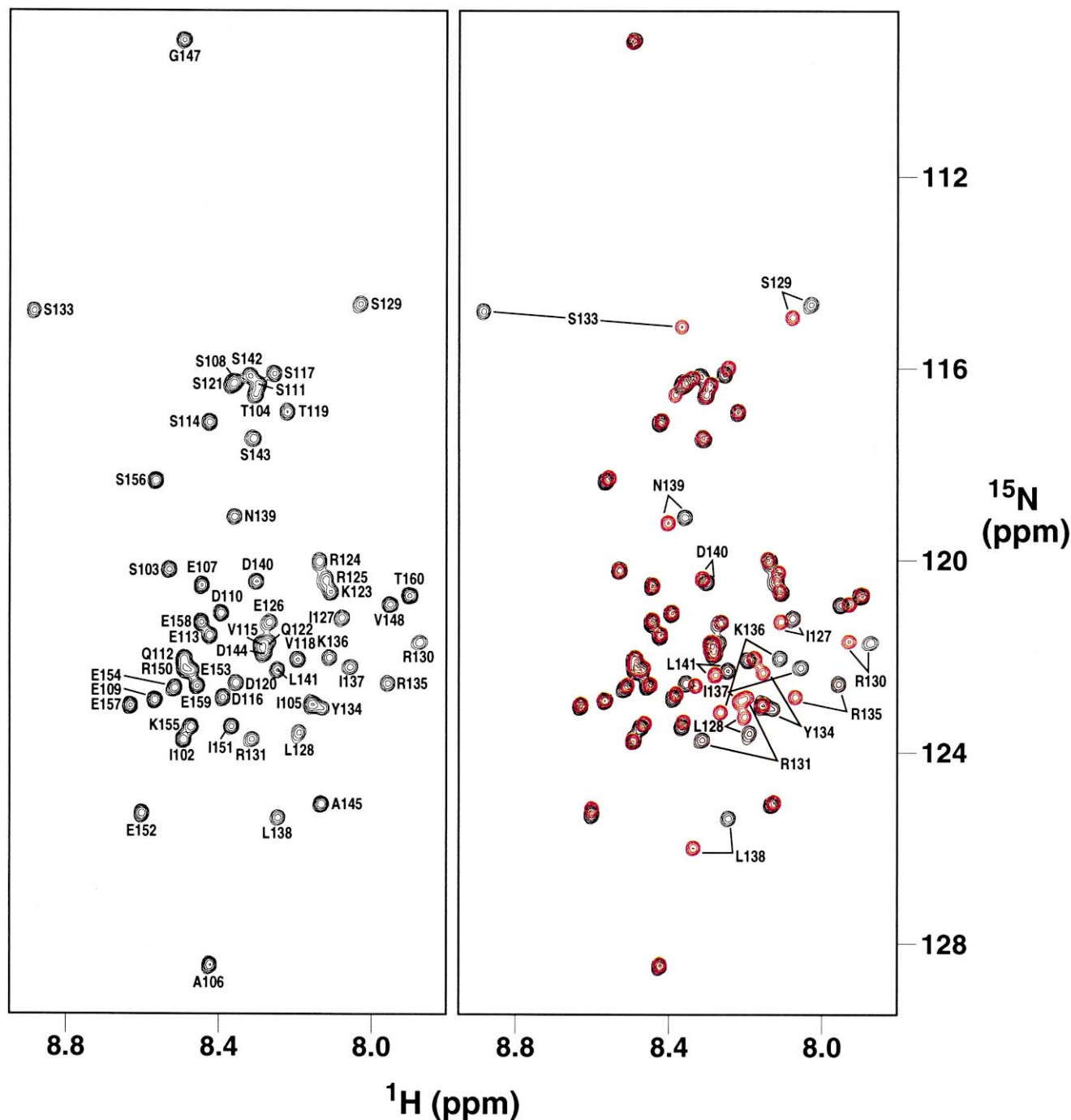
Fig. 1. a: ^1\text{H} - ^{15}\text{N} HSQC spectrum of Ser 133 -phosphorylated KID recorded under conditions described in the text. Residue-specific assignments are indicated. b: An overlay of the ^1\text{H} - ^{15}\text{N} HSQC spectra of Ser 133 -phosphorylated (black) and non-phosphorylated (red) forms of KID. Residues affected by Ser 133 phosphorylation are labeled.
